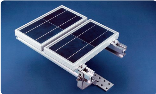
Patented Profilink system: The flexible solution for installing framed and frameless modules on pitched roofs.
