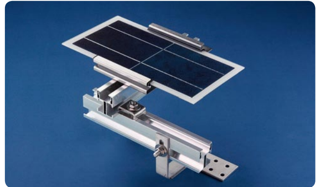
Patented Profilink system: The flexible solution for installing framed and frameless modules on pitched roofs.
